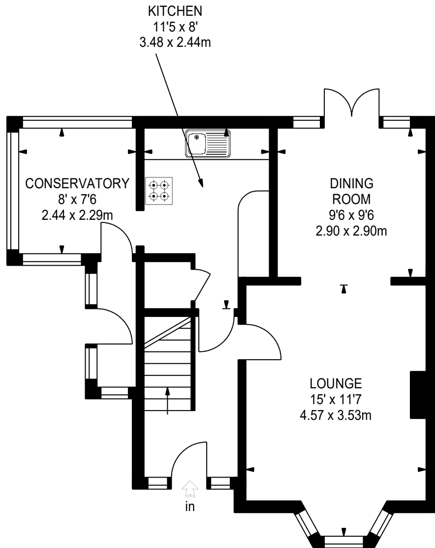
GROUND FLOOR
